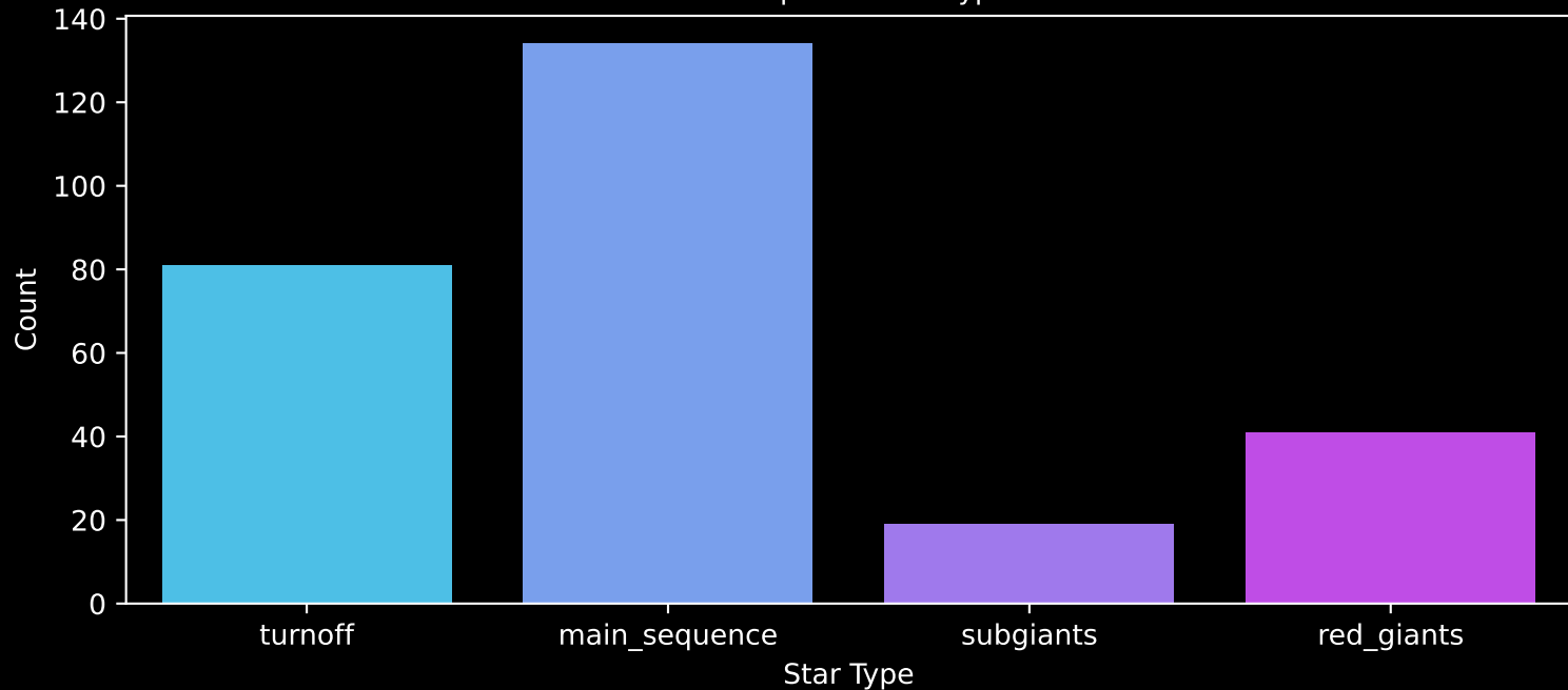
GALAH DR4 Field: [458] Count plot of Star Type
