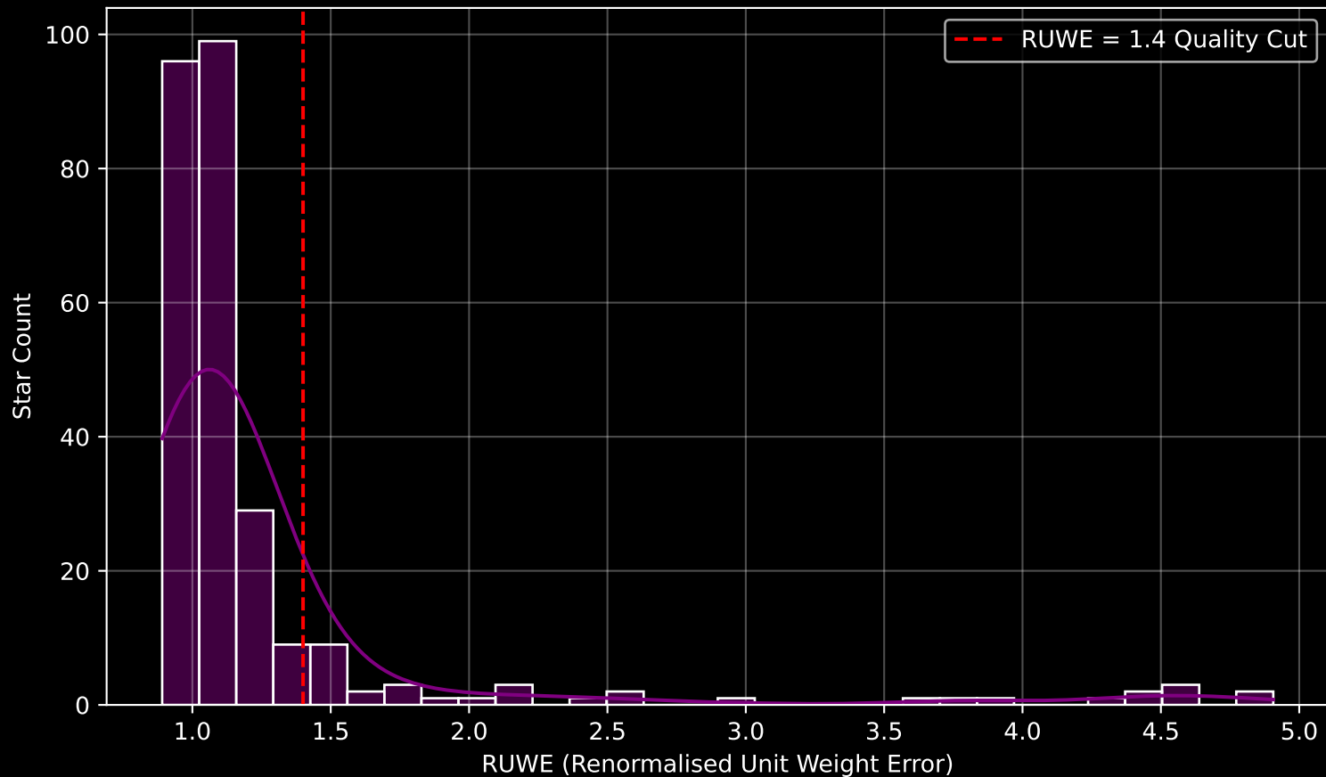
GALAH DR4 Field [458] RUWE Distribution (n= 267)
