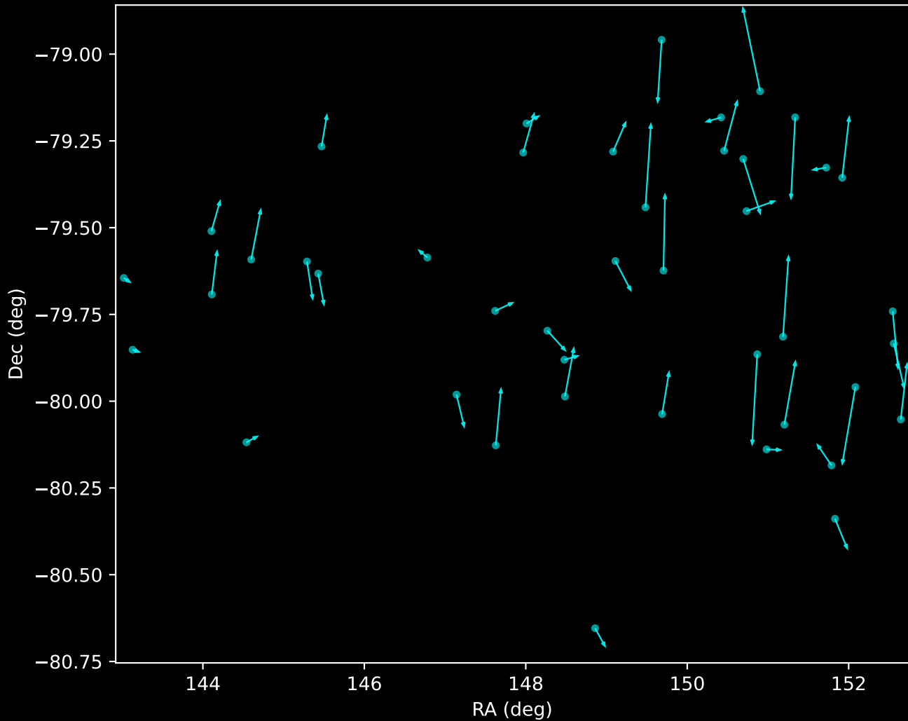
GALAH DR4 Noise Stream Proper Motion Vectors (n=43)
