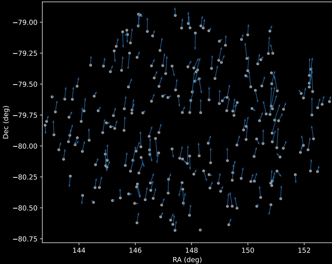
GALAH DR4 Cluster 0 Proper Motion Vectors (n=227)
